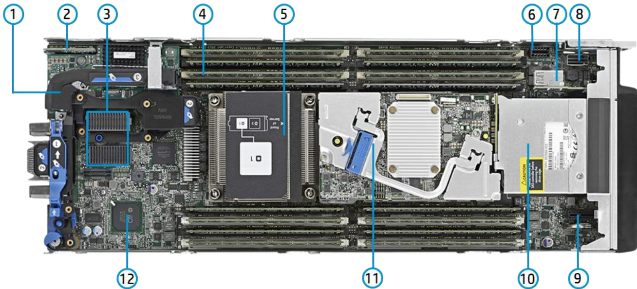
HP ProLiant WS460c Gen9 Graphics Server Blade – Internal View
